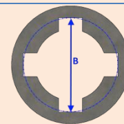
Reach maximum diameter of the cutter with the sample centered -B: Without bar guide -B': With bar guide
