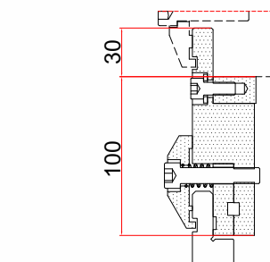
Euro American Type Mechanical Punch Clamping
