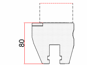
Wila Hydraulic New Standard Automatic Punch Clamping
